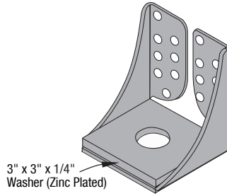
QGCW for Threaded Rods
