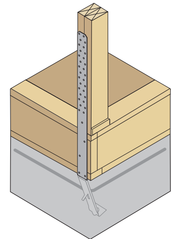
Rim Joist Installation at Corner
