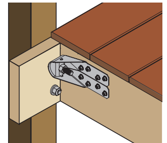
HDTT as Deck Tension Tie
