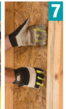
7 Check the tension on the installed cables
