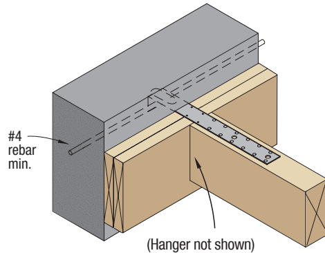
Purlin-to-Wall Attachment
