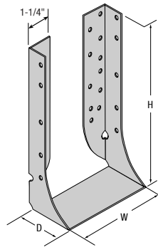
TYPICAL INVERTED FLANGE (IF) U HANGERS
