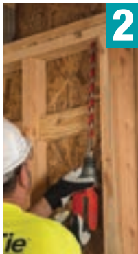
Drill top hole through the plate
