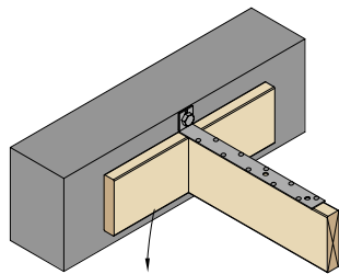
LTT20 as Tension Tie
