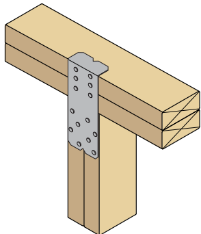
RSPT6-2 to Double Top Plate Installation
