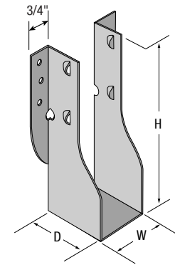
TYPICAL U HANGERS
