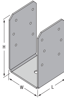
POST BASE STRAP
