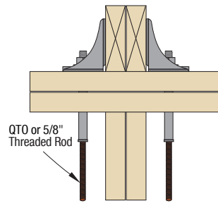
QGC (back-to-back) for 2-ply truss/rafter
