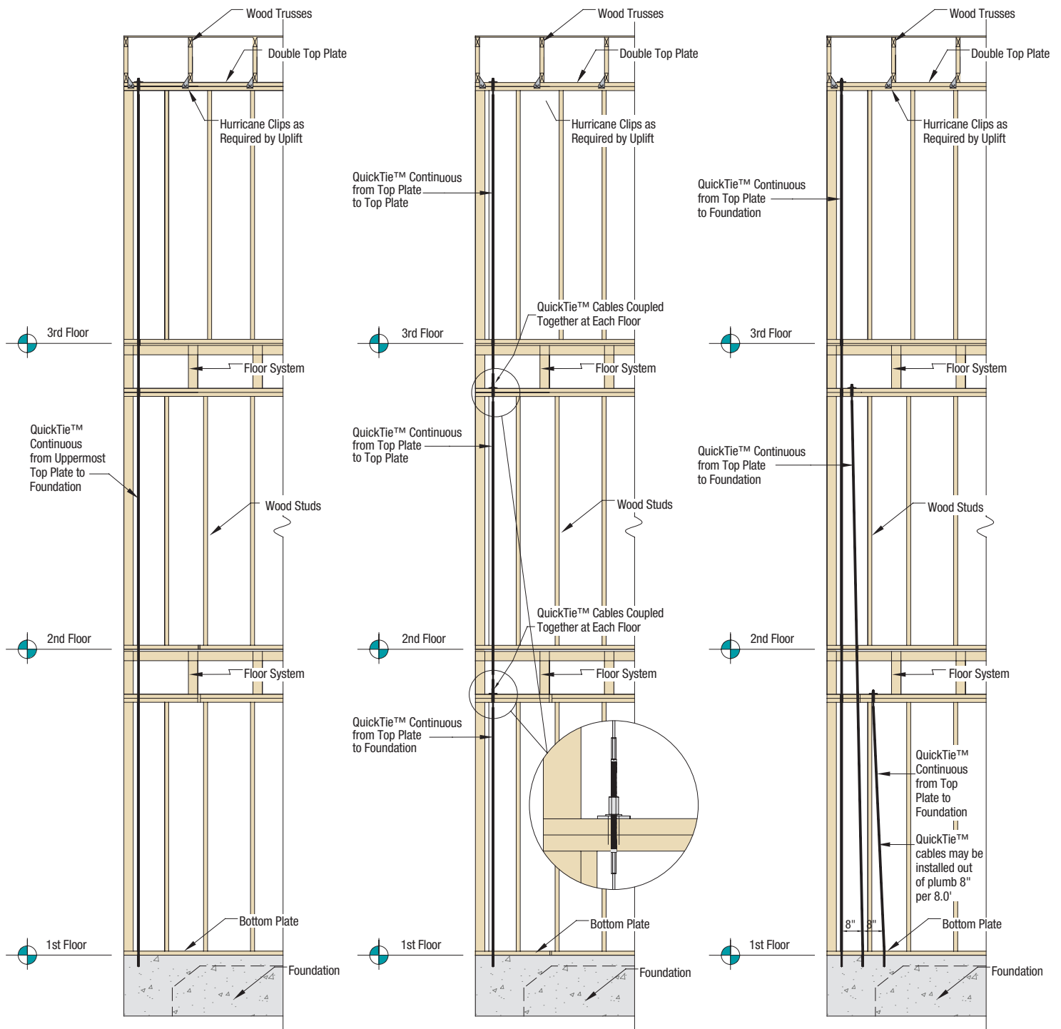
OPTION 1 (Typical) [Single QuickTie™ Cables Connected from Roof Level to Foundation]
