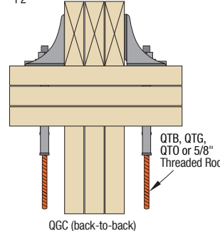
QGC (back-to-back) for 3-ply truss/rafter
