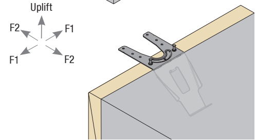
Installation for sill plate and studs
