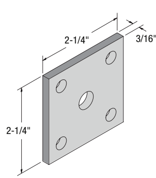
BPBC2.25-33N (QTB) BPBC2.25-33NS (QTB)
