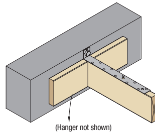
LTT20 as Tension Tie
